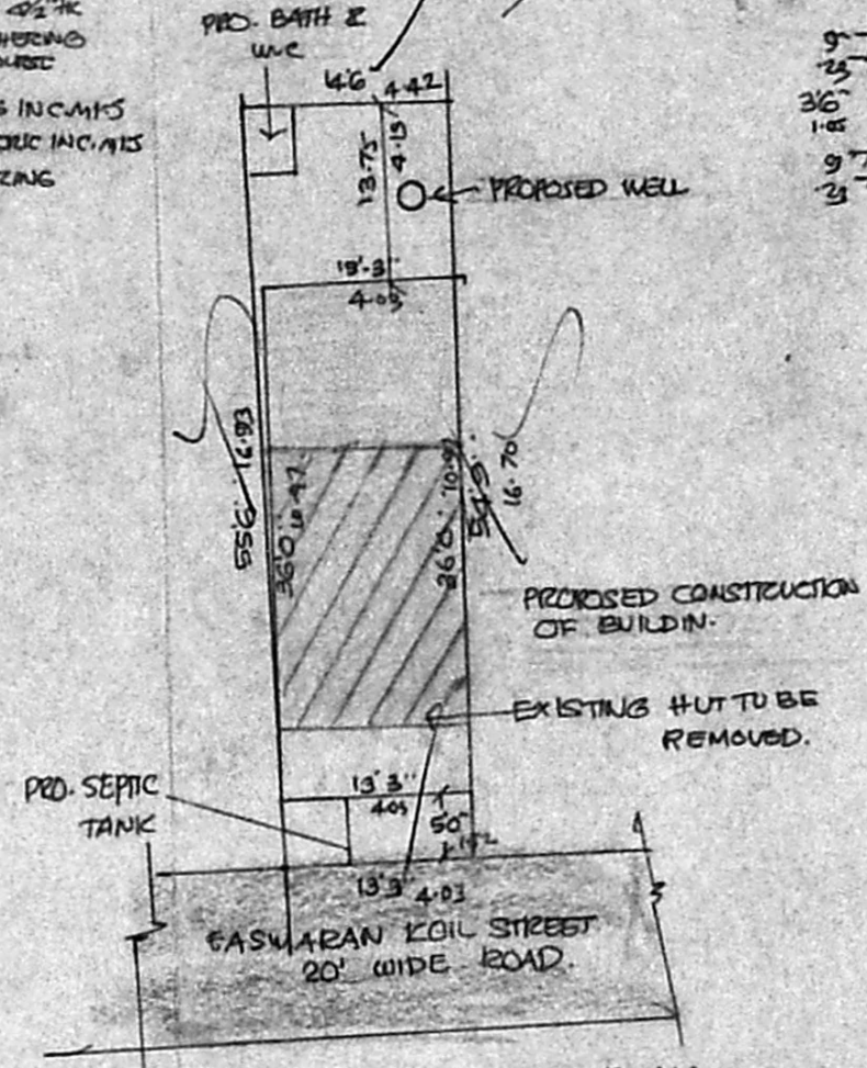
SITE PLAN SCALE 1 INCH = 16 FEET OR 1:200
